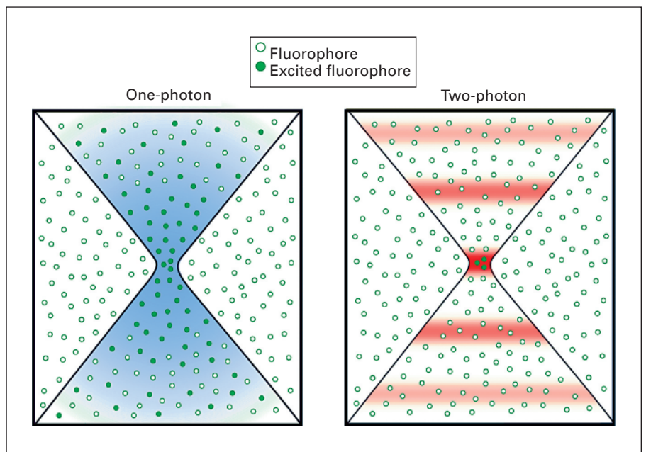
Fig. 2. Fluorescence excitation for one- and two-photon microscopy. In confocal microscopy, a continuous wave ultraviolet or visible light laser excites fluorophores throughout the volume. In two-photon microscopy, an infrared laser provides pulsed illumination such that the density of photons sufficient for simultaneous absorption of two photons by fluorophores only occurs at the focal point.
