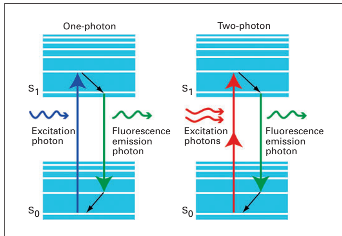
Fig. 1. Jablonski diagram demonstrating one- and two-photon fluorescence excitation. Two-photon excitation results from the simultaneous absorption of two low-energy photons by a fluorophore.
